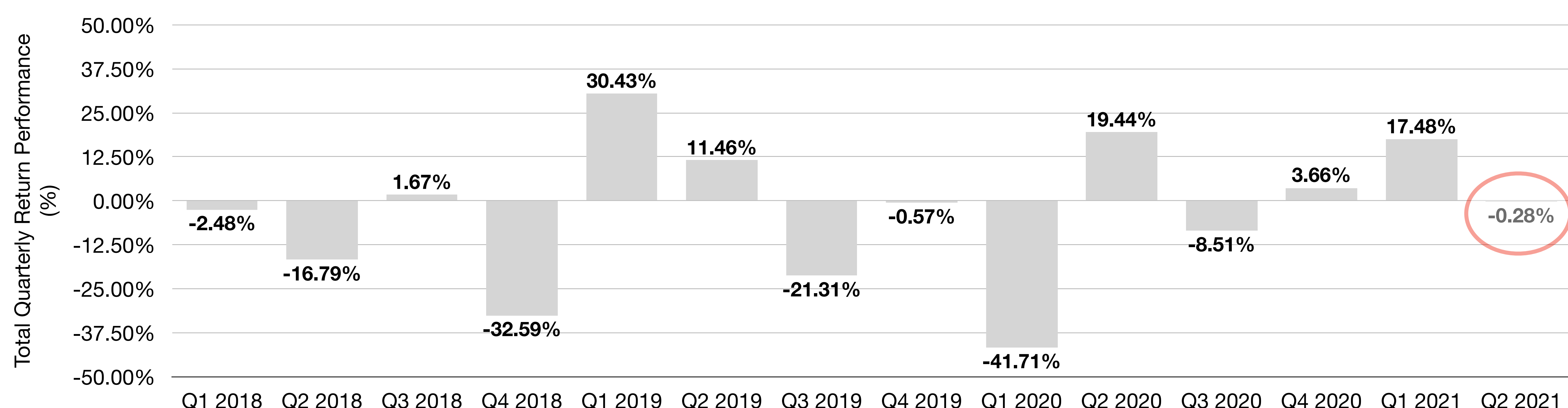
CROWDBUREAU PEER-TO-PEER LENDING AND EQUITY CROWDFUNDING INDEX PERFORMANCE (CBP2PTR) Quarterly Total Return Performance January 1, 2018 through June 30, 2021
